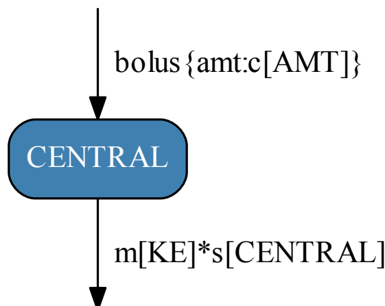
Fig. 1.3: One compartment model with bolus dosing for Tut Script . Here c[AMT] is the amount of the bolus dose. m[KE] is the elimination rate and s[CENTRAL] is the current amount in the central compartment.
