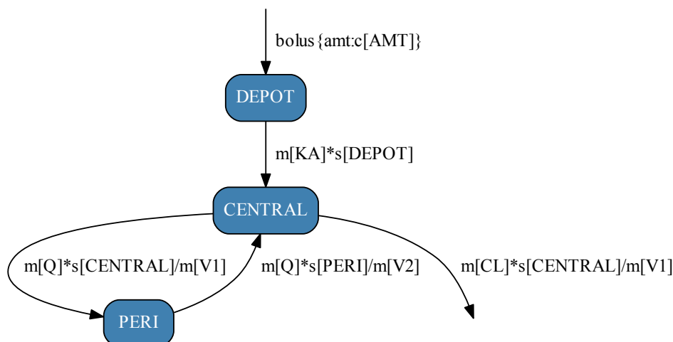
Fig. 4.3: Two compartment model with depot dosing for Gen Script . This is the same model as Fig. 4.1.
